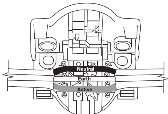
Mid connection
