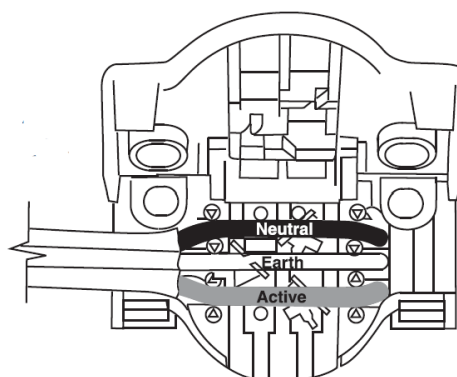
End connection
